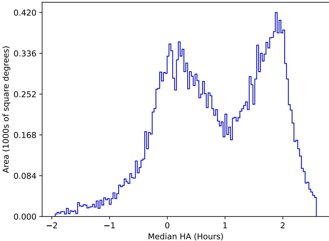
too_elab_r64_d2_griz_v3.4_10yrs All sky u band: Median HA
