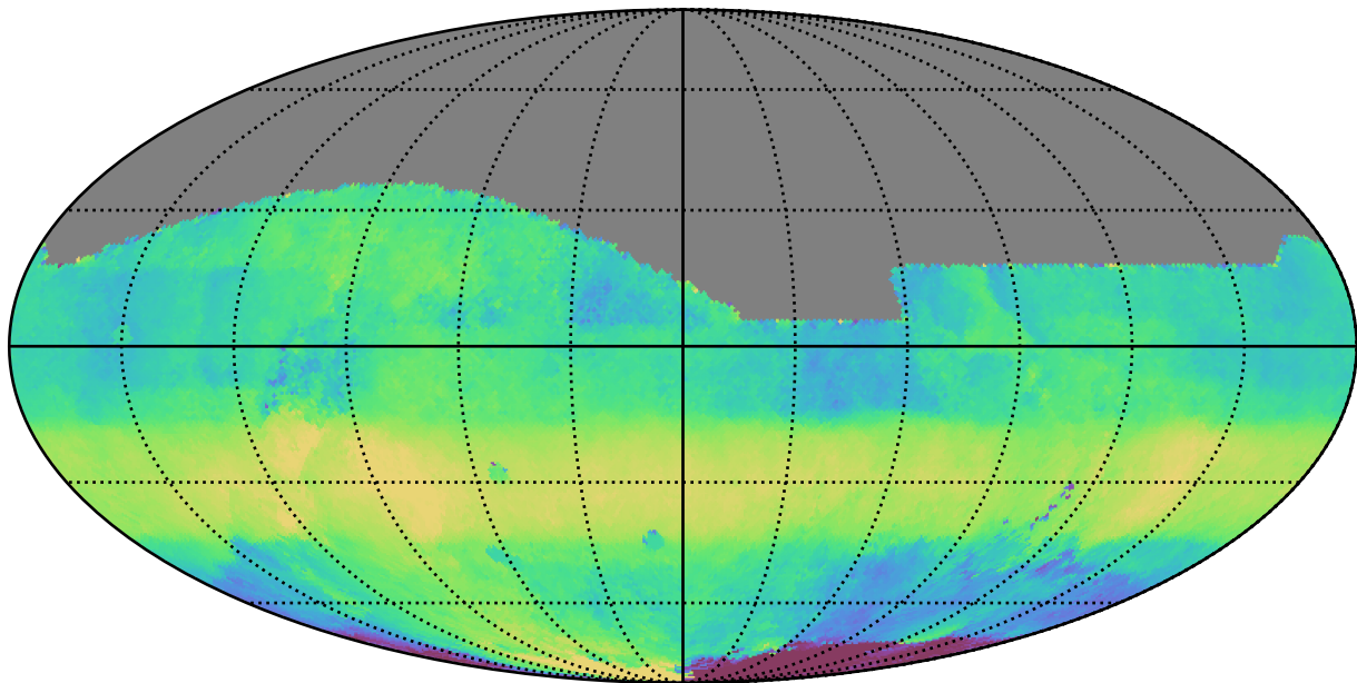
too_elab_r64_d2_griz_v3.4_10yrs All sky r band: Median HA
