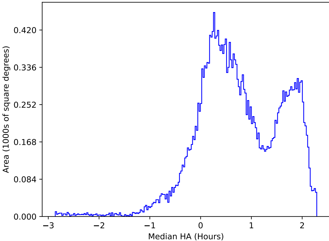
too_elab_r64_d2_griz_v3.4_10yrs All sky r band: Median HA
