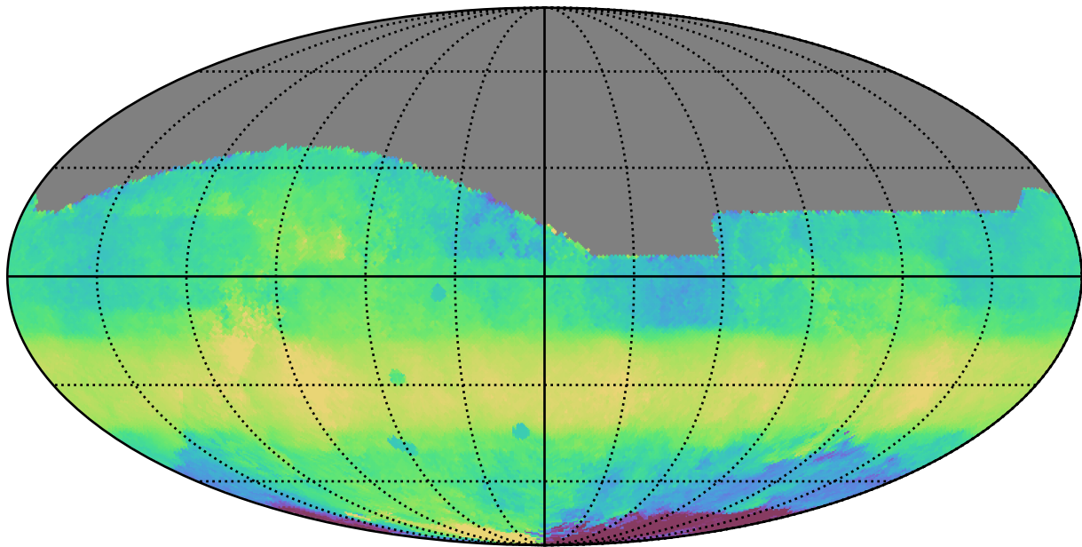
too_elab_r64_d2_griz_v3.4_10yrs All sky i band: Median HA
