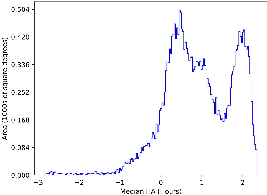
too_elab_r64_d2_griz_v3.4_10yrs All sky i band: Median HA
