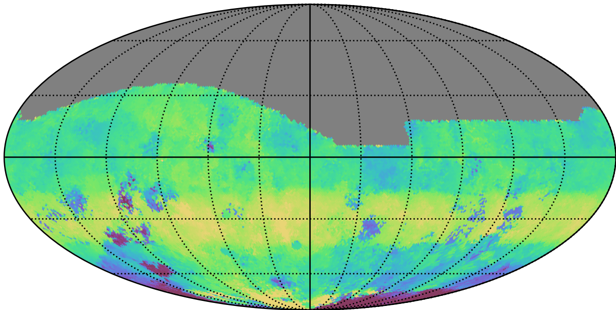
too_elab_r64_d2_griz_v3.4_10yrs All sky g band: Median HA
