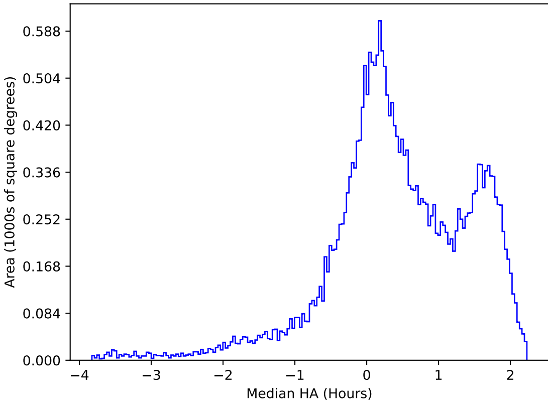
too_elab_r64_d2_griz_v3.4_10yrs All sky g band: Median HA
