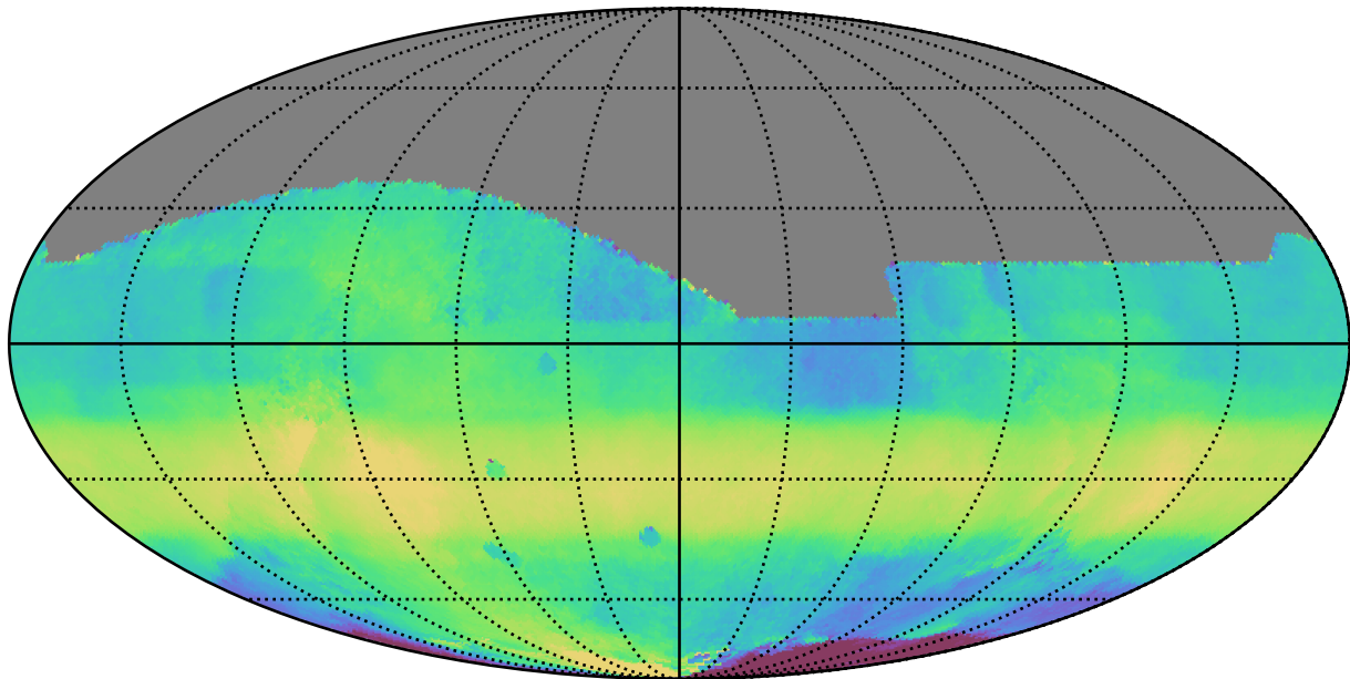
too_elab_r64_d2_griz_v3.4_10yrs All sky all bands: Median HA
