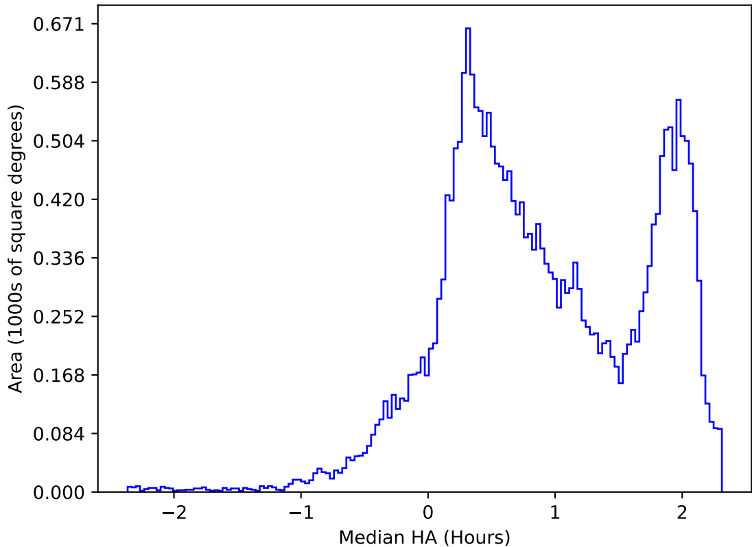
too_elab_r64_d2_griz_v3.4_10yrs All sky all bands: Median HA
