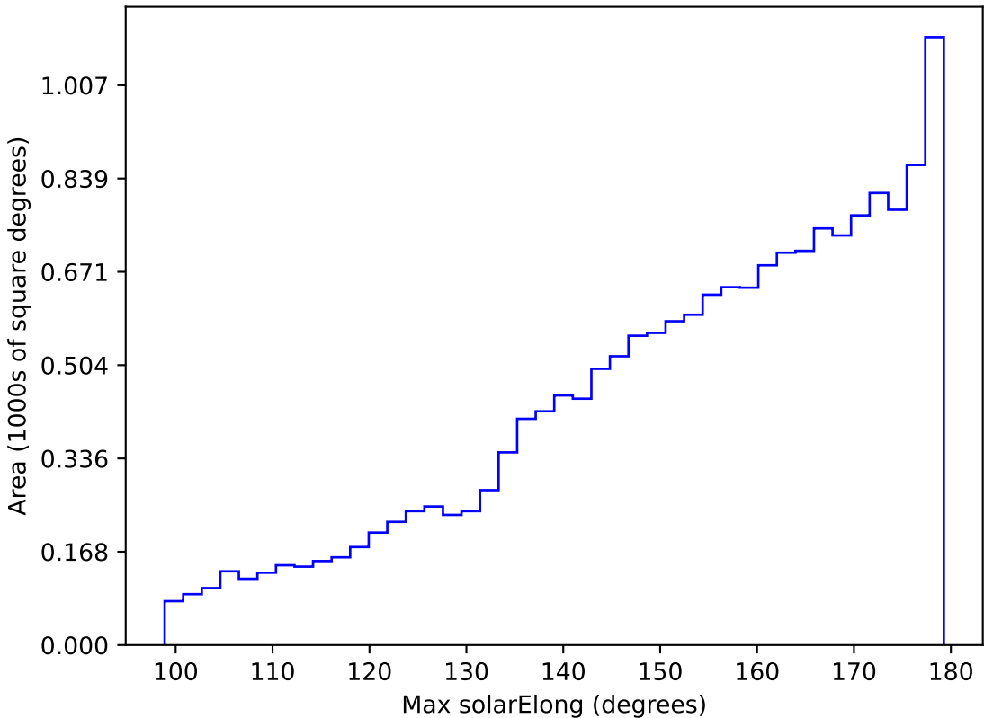
too_elab_r64_d2_griz_v3.4_10yrs WFD z band: Max solarElong
