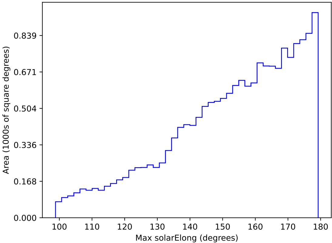
too_elab_r64_d2_griz_v3.4_10yrs WFD y band: Max solarElong
