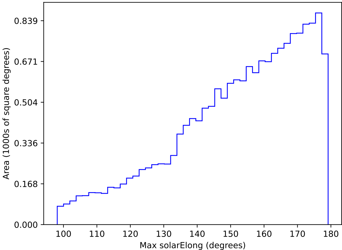
too_elab_r64_d2_griz_v3.4_10yrs WFD u band: Max solarElong
