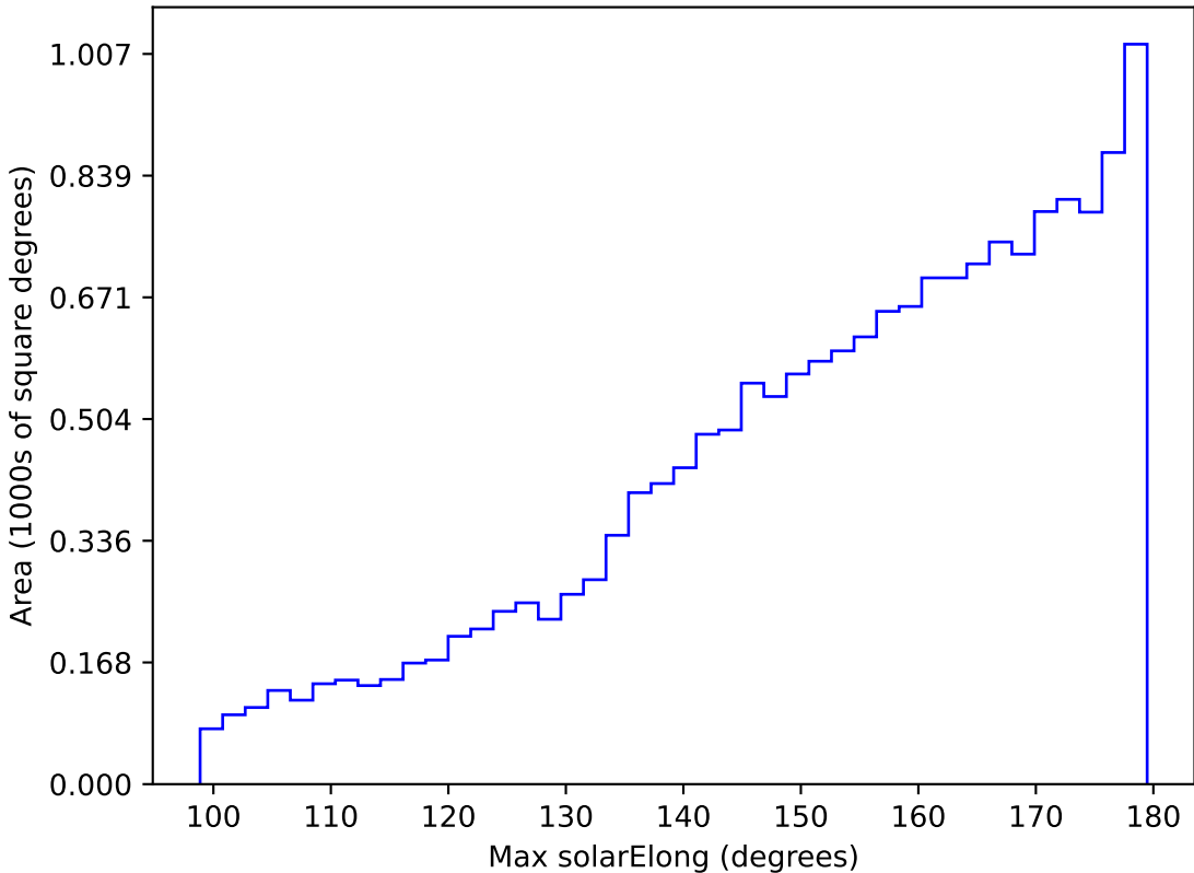
too_elab_r64_d2_griz_v3.4_10yrs WFD r band: Max solarElong
