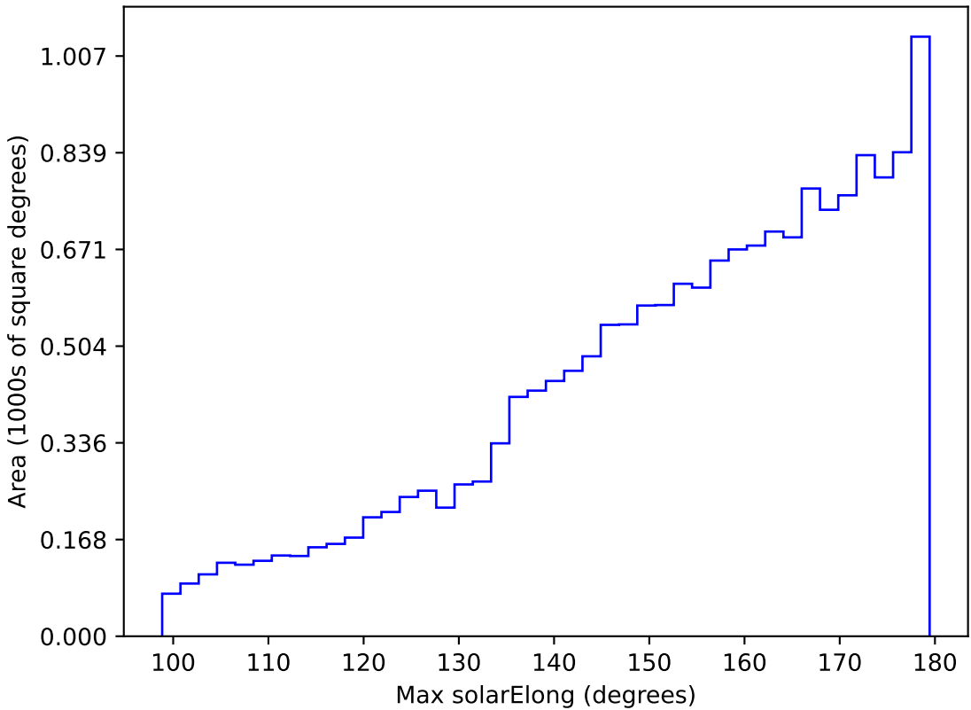
too_elab_r64_d2_griz_v3.4_10yrs WFD i band: Max solarElong
