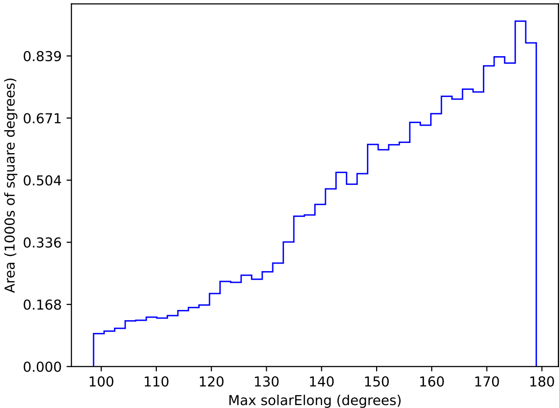
too_elab_r64_d2_griz_v3.4_10yrs WFD g band: Max solarElong
