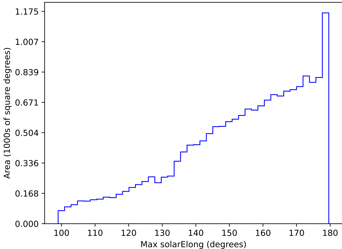
too_elab_r64_d2_griz_v3.4_10yrs WFD all bands: Max solarElong
