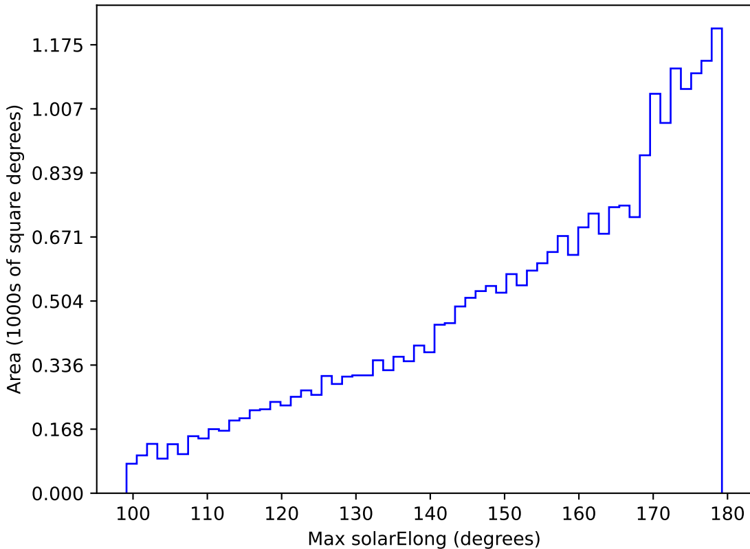
too_elab_r64_d2_griz_v3.4_10yrs All sky z band: Max solarElong
