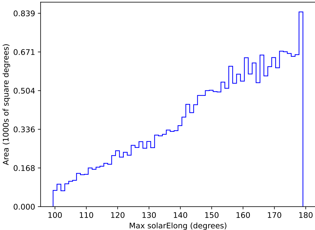
too_elab_r64_d2_griz_v3.4_10yrs All sky y band: Max solarElong
