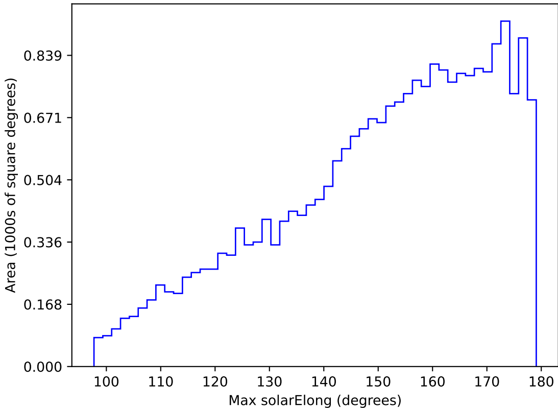
too_elab_r64_d2_griz_v3.4_10yrs All sky u band: Max solarElong
