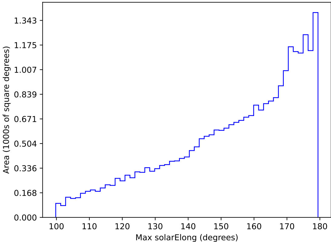
too_elab_r64_d2_griz_v3.4_10yrs All sky r band: Max solarElong
