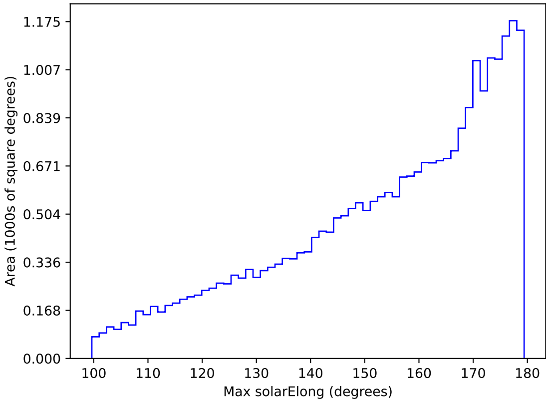
too_elab_r64_d2_griz_v3.4_10yrs All sky i band: Max solarElong
