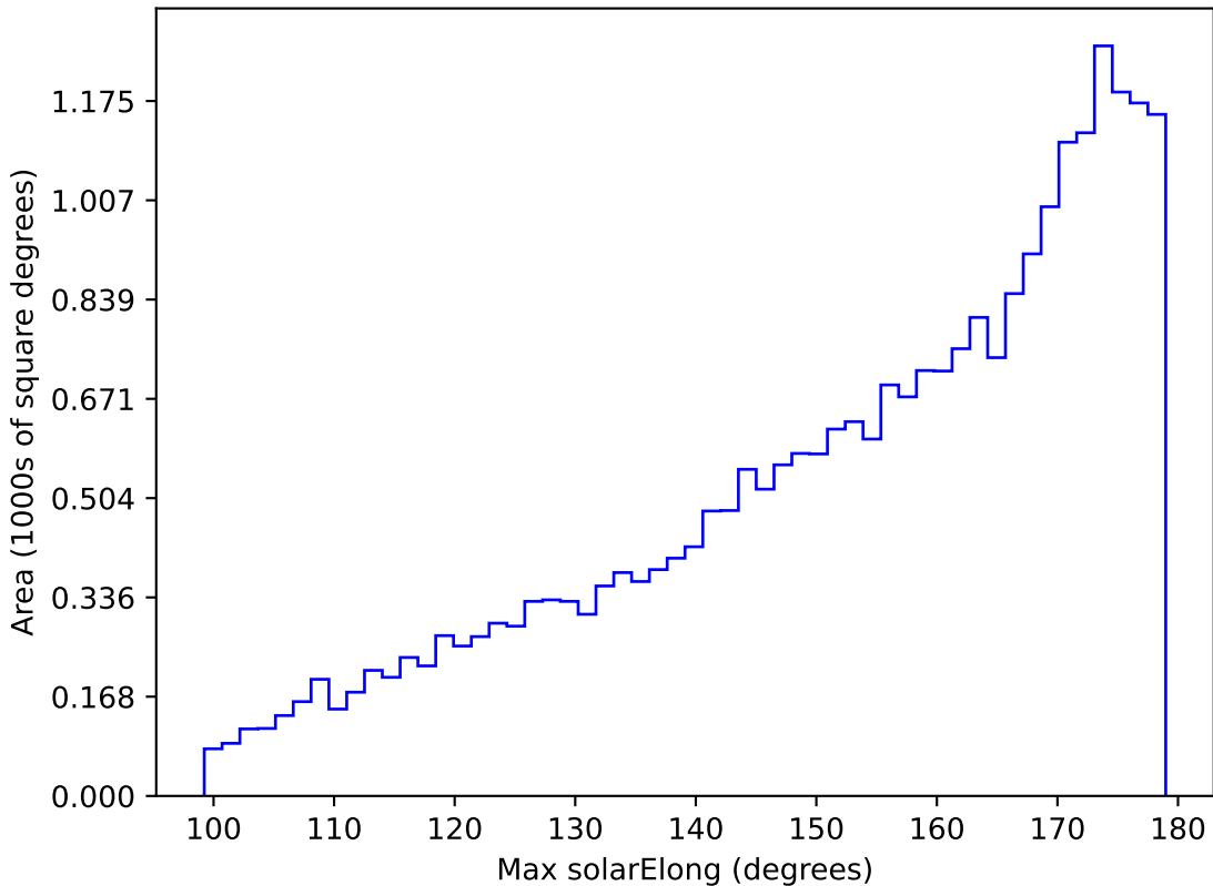
too_elab_r64_d2_griz_v3.4_10yrs All sky g band: Max solarElong
