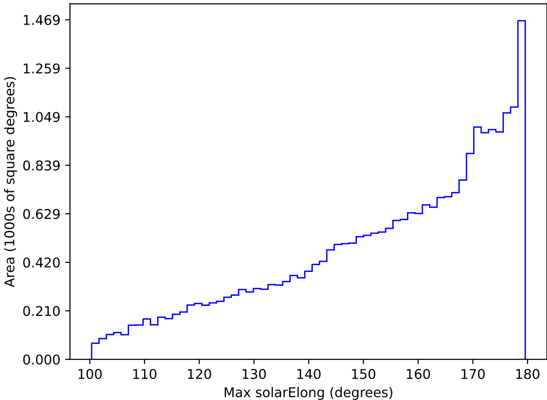
too_elab_r64_d2_griz_v3.4_10yrs All sky all bands: Max solarElong
