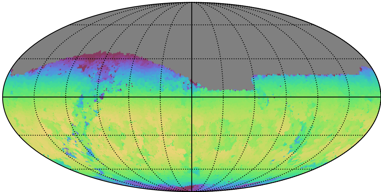
too_elab_r64_d2_griz_v3.4_10yrs Yr 1 z band: Max skyBrightness
