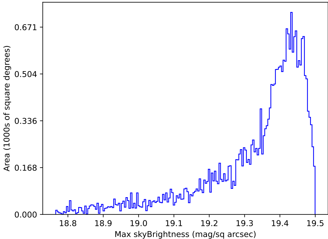
too_elab_r64_d2_griz_v3.4_10yrs Yr 1 z band: Max skyBrightness
