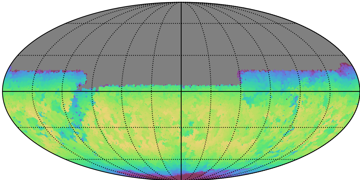
too_elab_r64_d2_griz_v3.4_10yrs Yr 1 y band: Max skyBrightness
