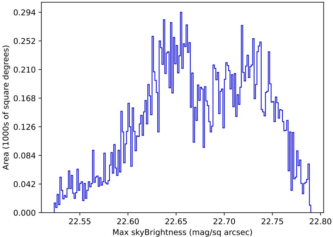
too_elab_r64_d2_griz_v3.4_10yrs Yr 1 u band: Max skyBrightness
