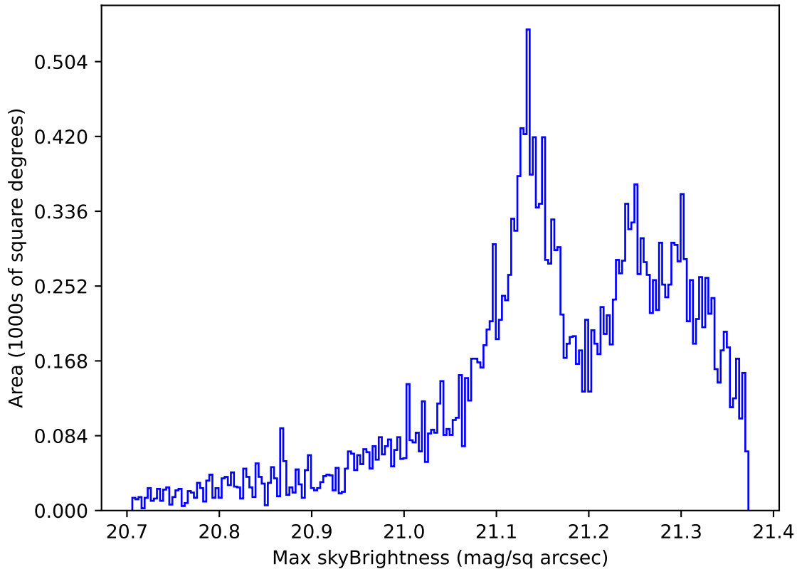
too_elab_r64_d2_griz_v3.4_10yrs Yr 1 r band: Max skyBrightness
