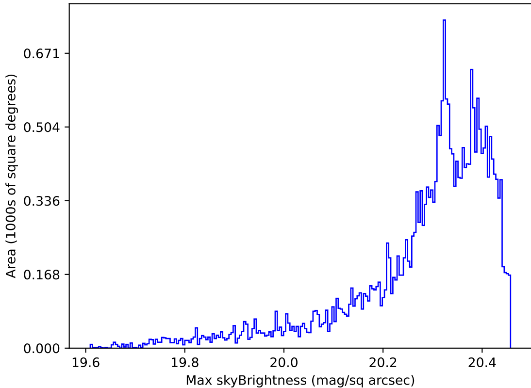
too_elab_r64_d2_griz_v3.4_10yrs Yr 1 i band: Max skyBrightness
