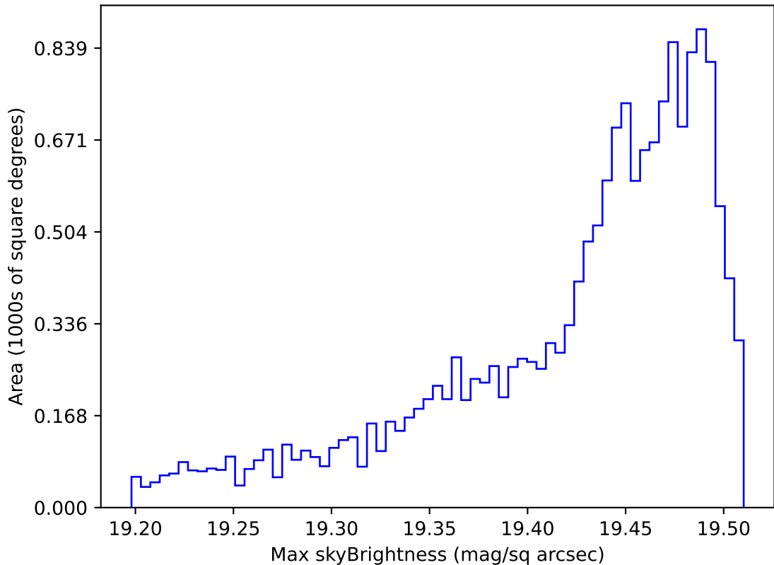
too_elab_r64_d2_griz_v3.4_10yrs WFD z band: Max skyBrightness
