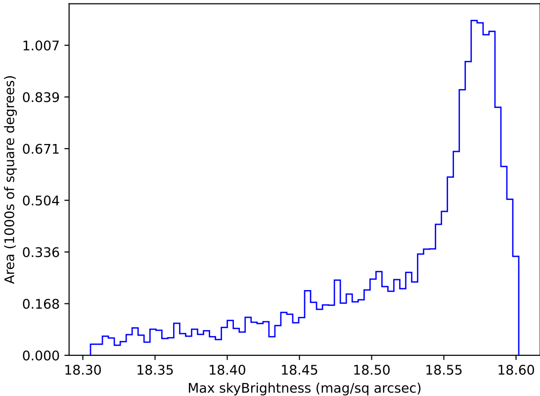
too_elab_r64_d2_griz_v3.4_10yrs WFD y band: Max skyBrightness
