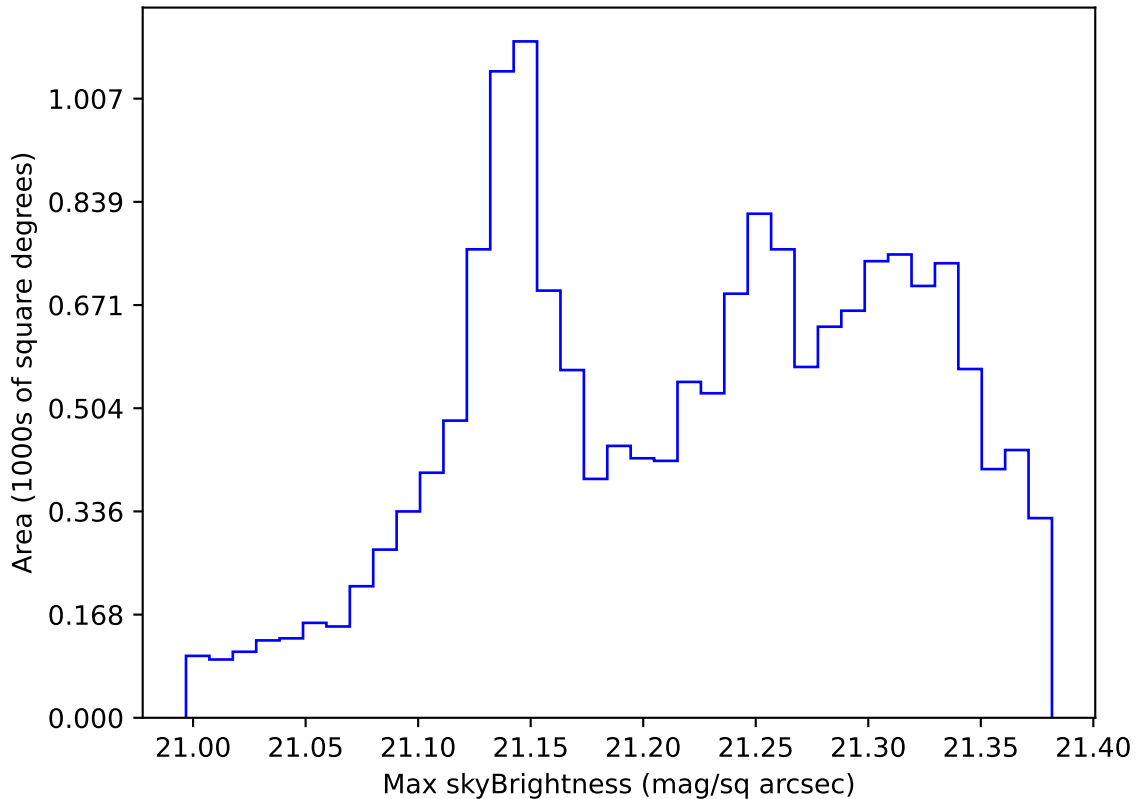
too_elab_r64_d2_griz_v3.4_10yrs WFD r band: Max skyBrightness
