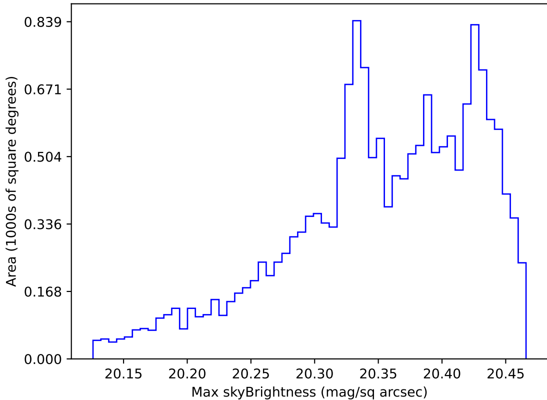
too_elab_r64_d2_griz_v3.4_10yrs WFD i band: Max skyBrightness
