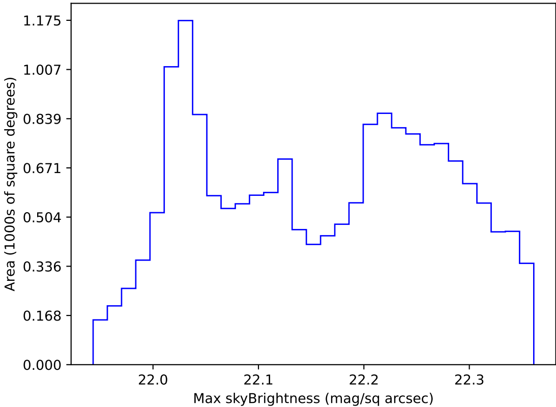
too_elab_r64_d2_griz_v3.4_10yrs WFD g band: Max skyBrightness
