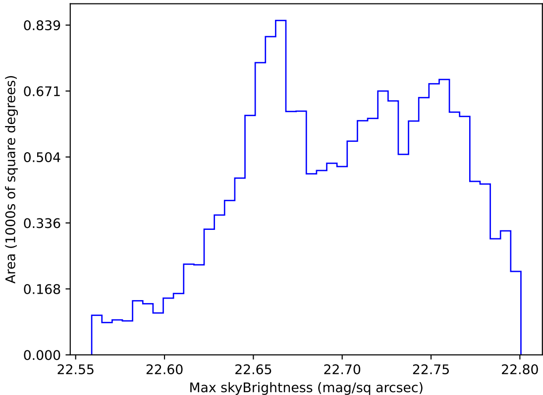
too_elab_r64_d2_griz_v3.4_10yrs WFD all bands: Max skyBrightness
