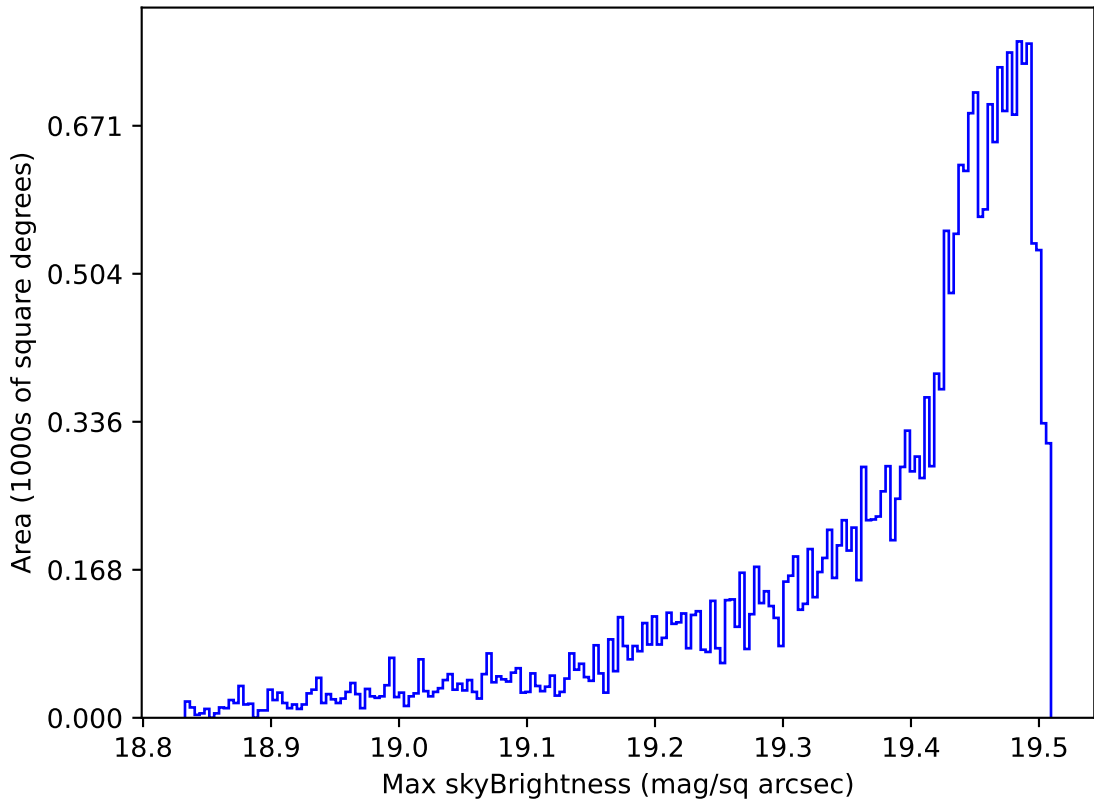
too_elab_r64_d2_griz_v3.4_10yrs All sky z band: Max skyBrightness
