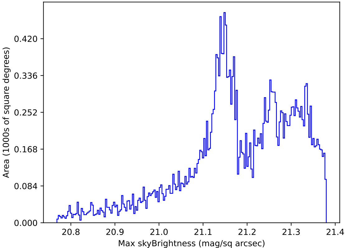
too_elab_r64_d2_griz_v3.4_10yrs All sky r band: Max skyBrightness
