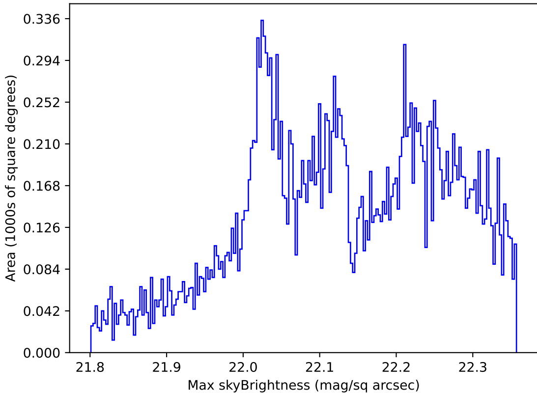
too_elab_r64_d2_griz_v3.4_10yrs All sky g band: Max skyBrightness
