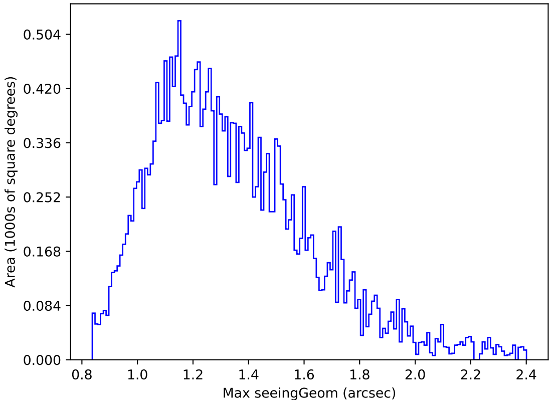
too_elab_r64_d2_griz_v3.4_10yrs Yr 1 r band: Max seeingGeom
