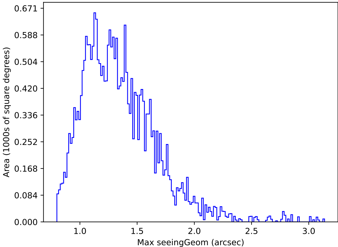
too_elab_r64_d2_griz_v3.4_10yrs Yr 1 g band: Max seeingGeom
