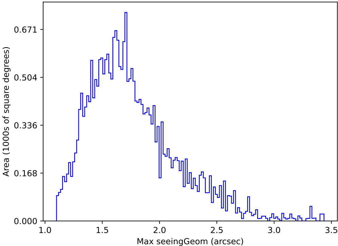
too_elab_r64_d2_griz_v3.4_10yrs Yr 1 all bands: Max seeingGeom
