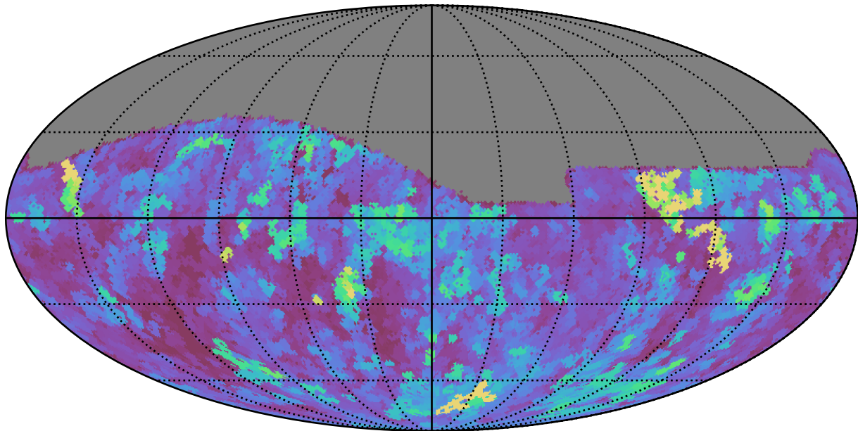
too_elab_r64_d2_griz_v3.4_10yrs Yr 1 all bands: Max seeingEff
