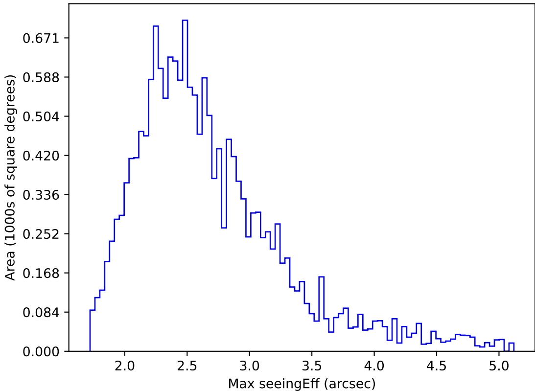
too_elab_r64_d2_griz_v3.4_10yrs WFD z band: Max seeingEff
