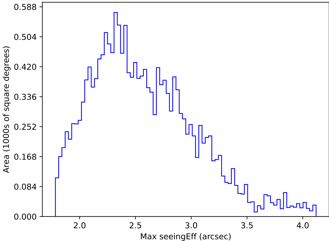
too_elab_r64_d2_griz_v3.4_10yrs WFD u band: Max seeingEff
