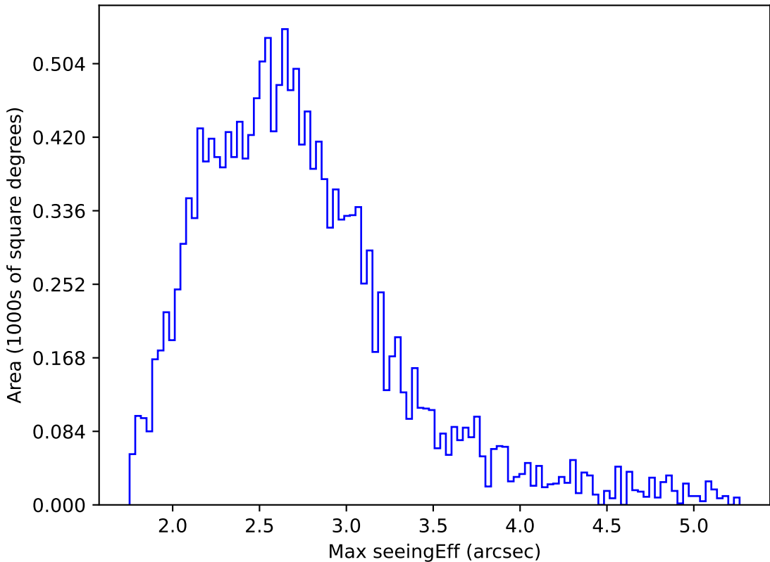
too_elab_r64_d2_griz_v3.4_10yrs WFD i band: Max seeingEff
