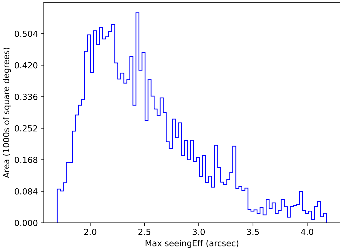
too_elab_r64_d2_griz_v3.4_10yrs WFD g band: Max seeingEff
