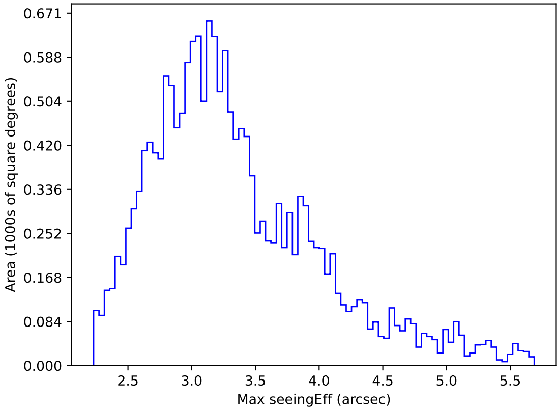
too_elab_r64_d2_griz_v3.4_10yrs WFD all bands: Max seeingEff
