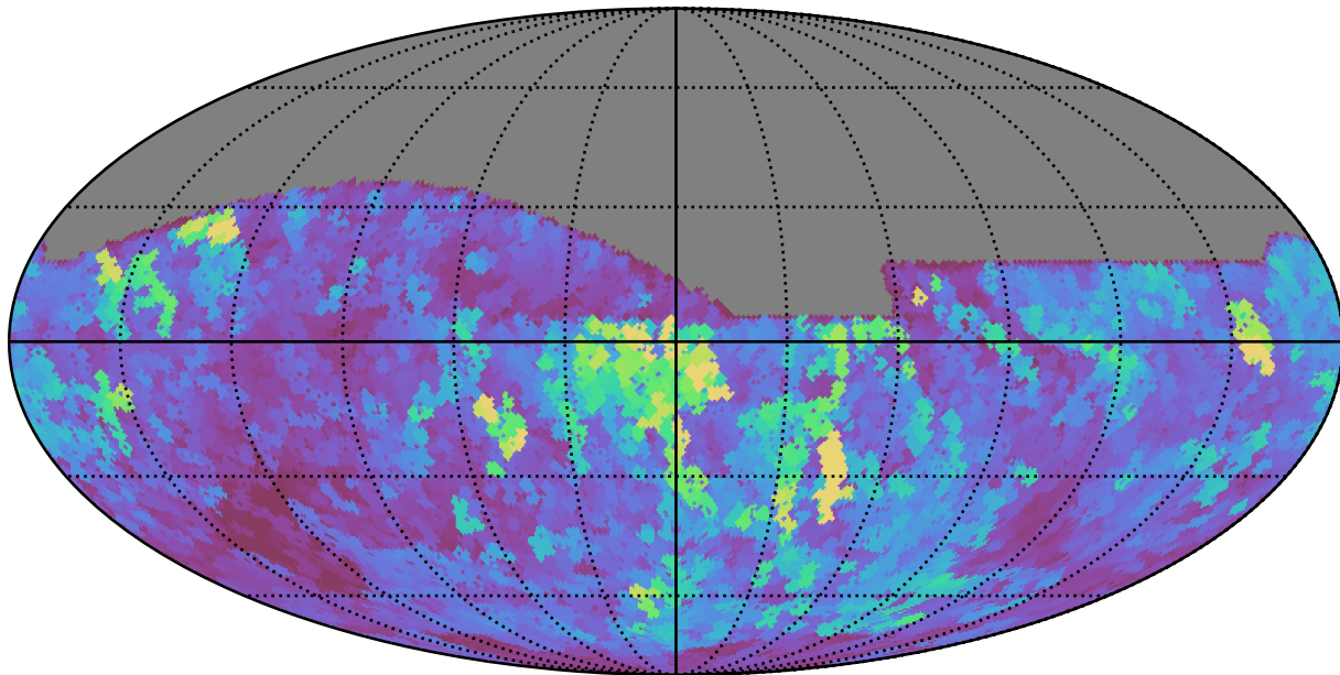
too_elab_r64_d2_griz_v3.4_10yrs All sky z band: Max seeingEff
