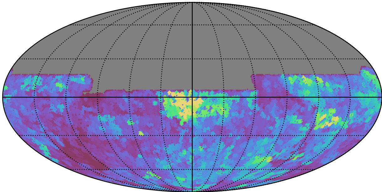
too_elab_r64_d2_griz_v3.4_10yrs All sky y band: Max seeingEff
