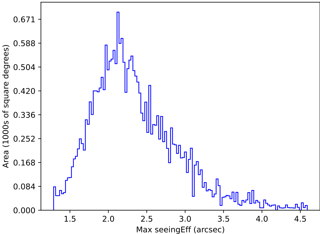
too_elab_r64_d2_griz_v3.4_10yrs All sky y band: Max seeingEff
